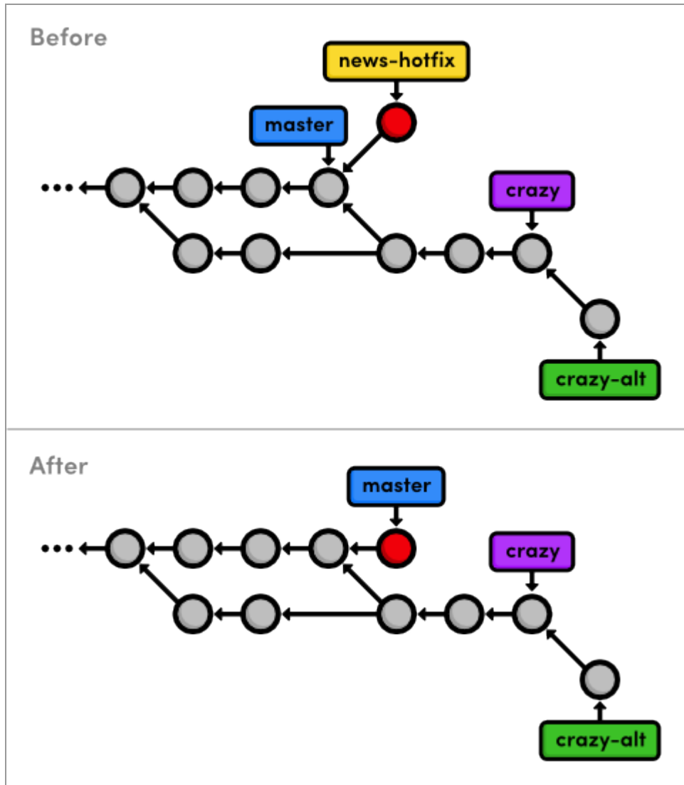
Fast-forwarding master to the news-hotfix branch
