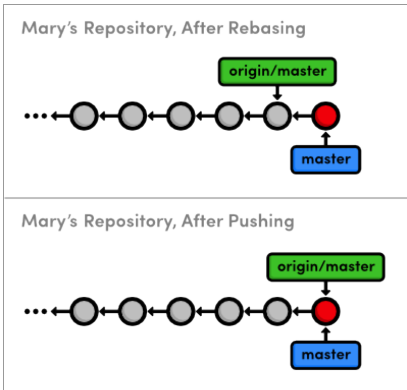
Updating the central repository's master
